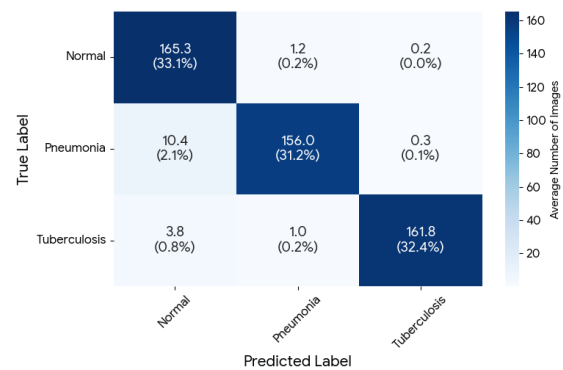
Figure 10. CNN Confusion matrix.
