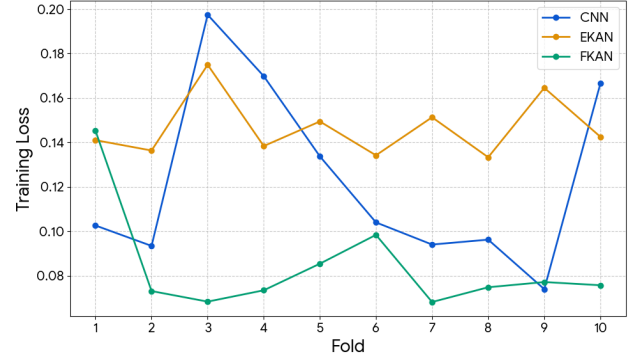
Figure 5. Loss values of training across folds.
