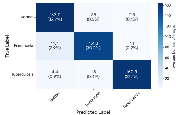
Figure 11. EKAN Confusion matrix.
