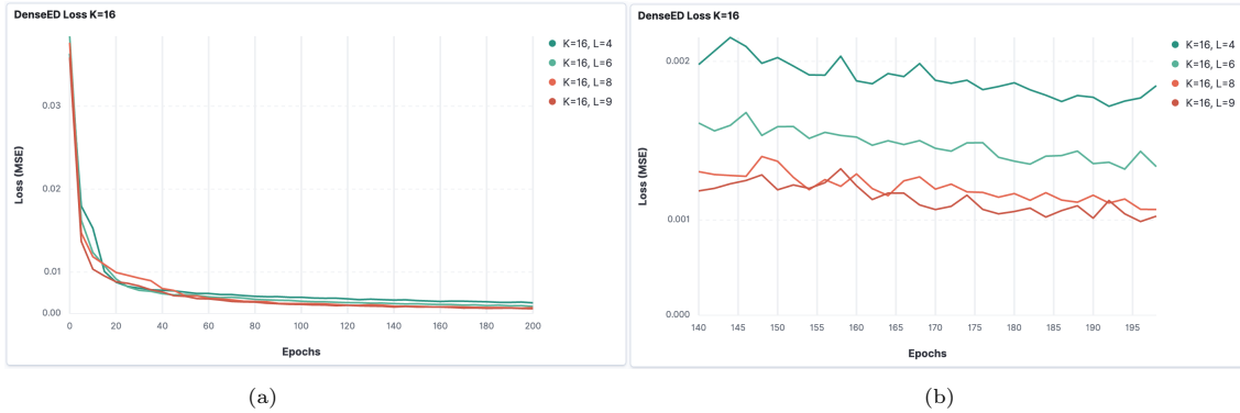
Fig. 9: (a) Graphical view of the training results of DenseED with k = 16 and l = (4, 6, 8, 9) (b) Zoomed view of the training results for DenseED with k = 16 and l = (4, 6, 8, 9) from epoch 140 to epoch 200.
