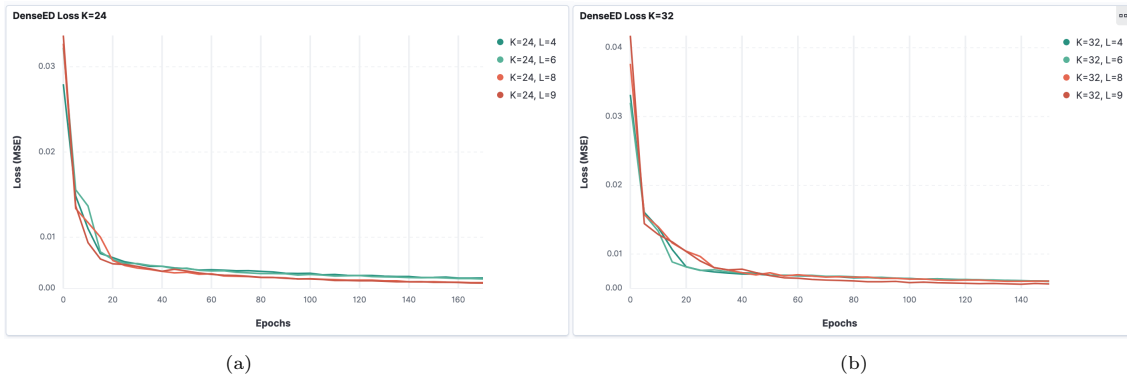
Fig. 10: (a) Graphical view of the training results of DenseED with k = 24 and l = (4, 6, 8, 9) (b) Graphical view of the training results of DenseED with k = 32 and l = (4, 6, 8, 9) .
