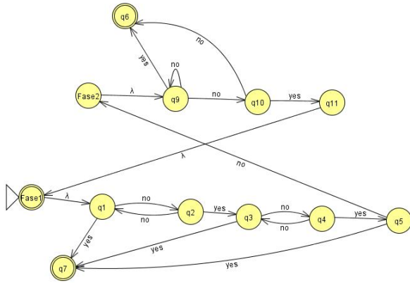
Figure 4. Automaton created to ViMeTGame storytelling.
