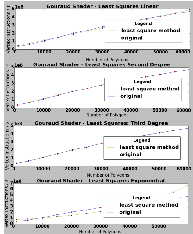
Figure 9. Automatic Adjustments: vertex shader
