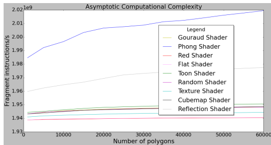
Figure 12. Fragment shader: curves comparison
